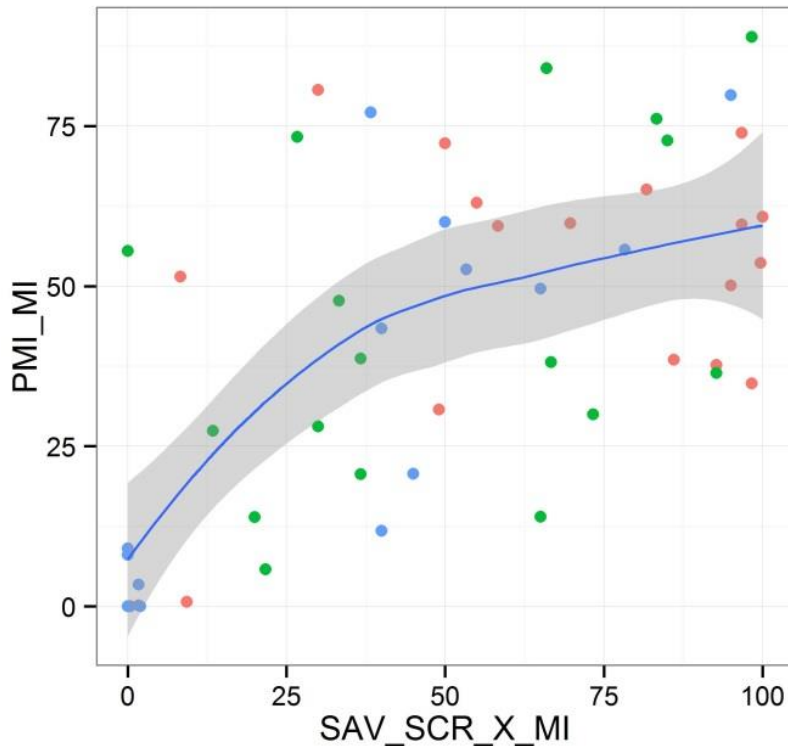
Figure 6. Scatterplot of PMI vs. SAV Index scores, with both indices scaled as MMIs.
