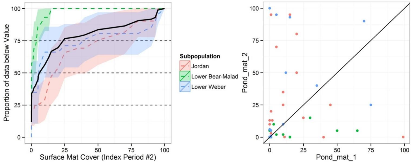
Figure 4. CDF for cover of Surface Mats during early-autumn sampling period (left), and scatterplot of Surface Mat cover (right) between summer (x-axis) and early-autumn (y-axis). Note that higher values of Surface Mat cover indicate a more degraded ecological state, while lower values of cover are preferred.
